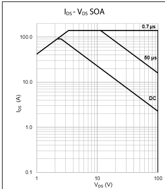
Figure 13: Safe Operating Area @ T_{case} = 25^\circ C
