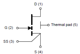
Circuit Symbol
